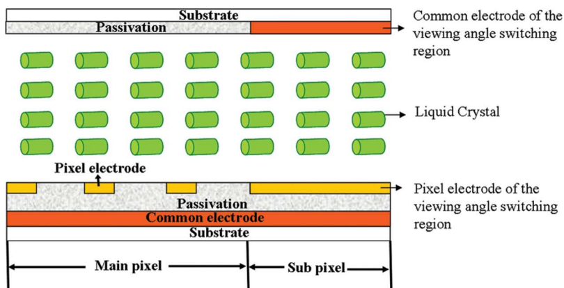
FIGURE 1 Schematic cell structure of the viewing angle controllable FFS-LCD.
