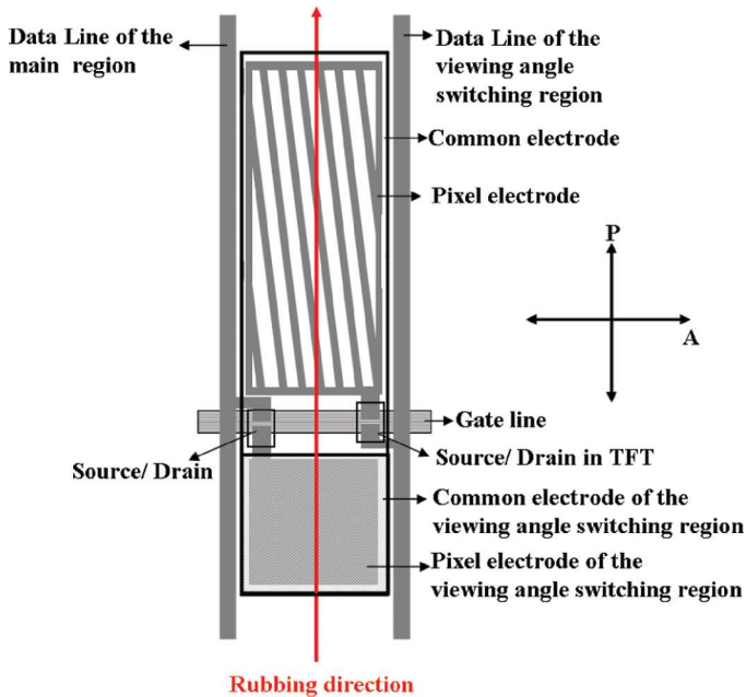
FIGURE 2 Top view of electrode structure of the viewing angle controllable FFS-LCD.
